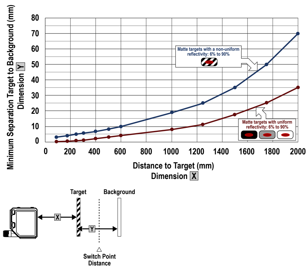
Figure 24. Minimum Object Separation Distance (90% to 6% reflectance)
